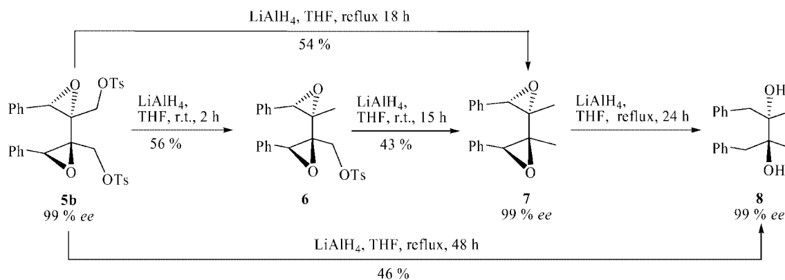
Scheme 3. Reduction of 5b .
