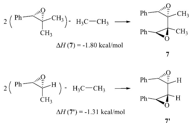
Scheme 6. Theoretical investigation of \pi – \pi stacking phenomena.
