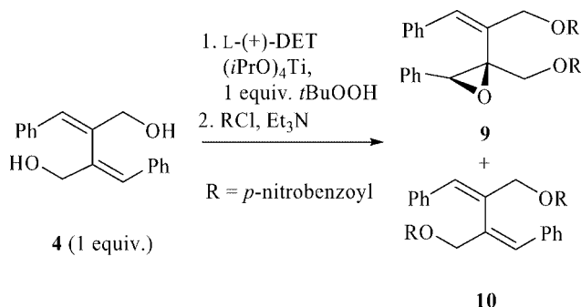
Scheme 4. Monoepoxidation of diallyl alcohol 4 .
