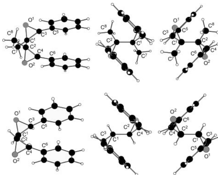
Figure 7. MP2/6-31G*-optimized structures of 7 (top) and 7' (bottom) in different views.
