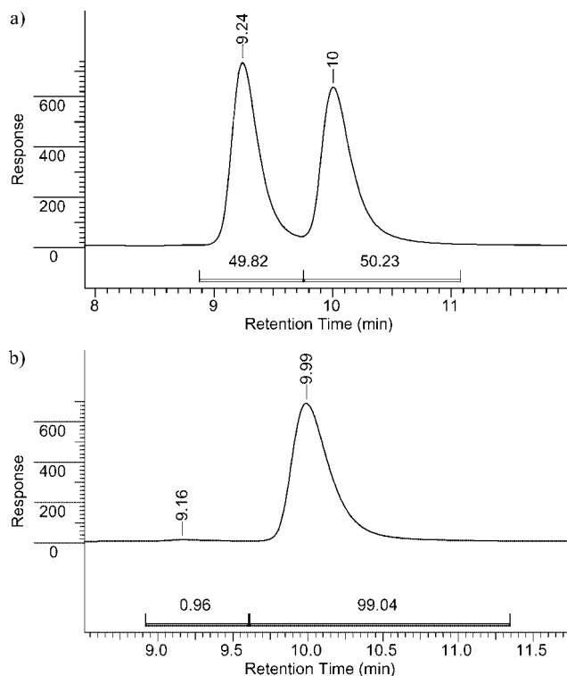
Figure 1. Chromatograms of: a) an approximately equimolar mixture of (all R )- 5a and (all S )- 5a , and b) the product of the asymmetric epoxidation [(all R )- 5a ]. Whelk( R,R ) column, eluent: n -hexane/ethanol 8:2, 0.8 mL min –1 .
