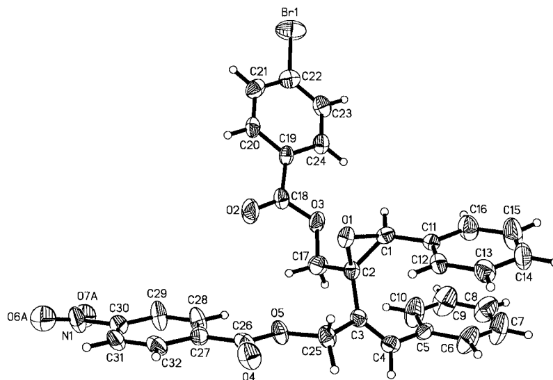
Figure 5. Molecular structure of 12 . The thermal ellipsoids correspond to 30% probability.
