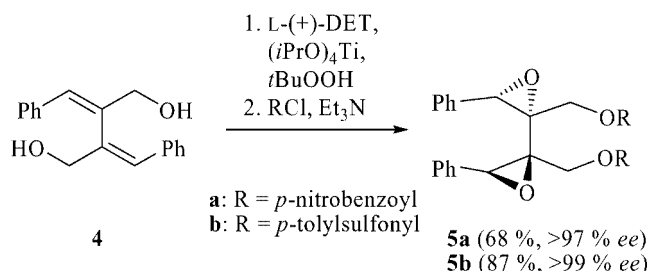
Scheme 2. Epoxidation of 4 and subsequent trapping of the product.
