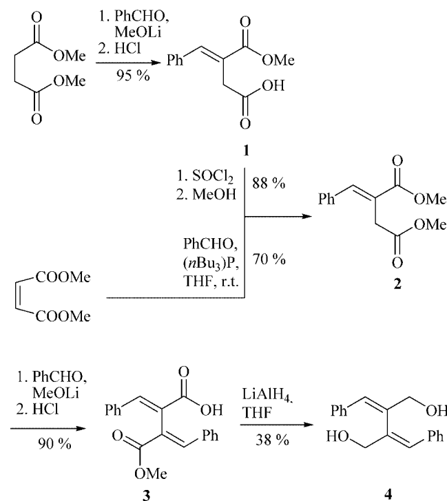
Scheme 1. Synthesis of diallyl alcohol 4 used as substrate in the Katsuki–Sharpless epoxidation.
