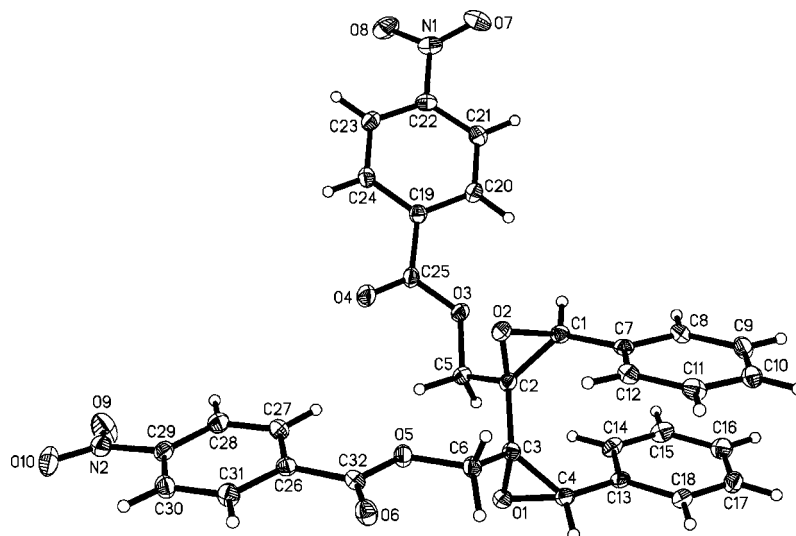
Figure 3. Molecular structure of 5a . The thermal ellipsoids correspond to 30% probability.
