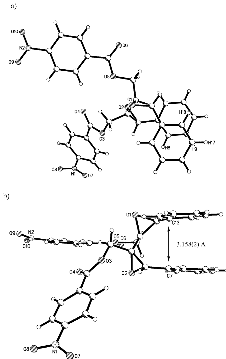
Figure 6. Different views of the structure of 5a .
