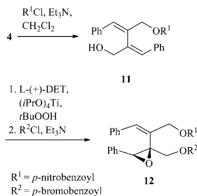
Scheme 5. Synthesis of a mixed diester monoepoxide.
