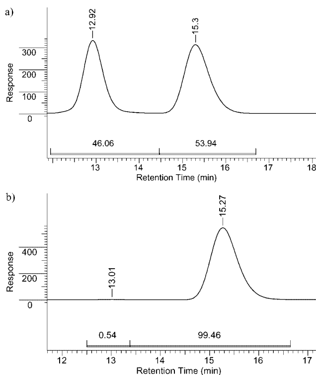
Figure 2. Chromatograms of: a) an approximately equimolar mixture of (all R )- 5b and (all S )- 5b , and b) the product of the asymmetric epoxidation [(all S )- 5b ]. Whelk( R,R ) column, eluent: n -hexane/ethanol 8:2, 0.8 mL min –1 .
